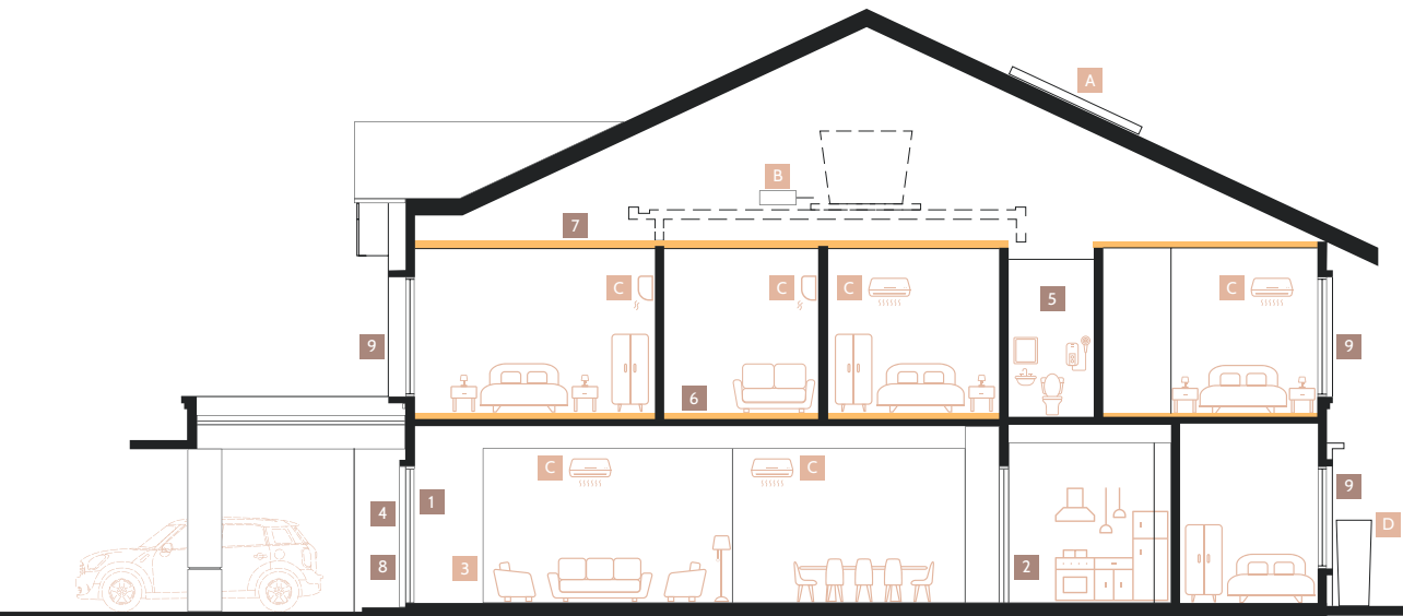
This diagram is for illustration purposes only and does not reflect the final position and design of the fittings.
